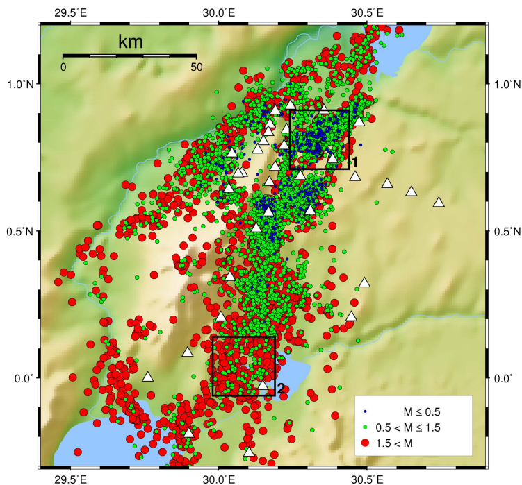
Fig. 10. Spatial distribution of the computed magnitudes. Coloured symbols represent different magnitude classes, see legend. White triangles indicate the station locations. Small events (green and blue symbols) could only be located in areas with high station density. This illustration is a clear indication that the apparent decrease of seismicity southwest of the Rwenzoris (cf. Fig. 2) is probably due to the lack of stations in this region. Two rectangles mark the areas where the magnitude-frequency relations presented in Fig. 11 were calculated.
