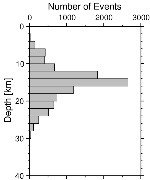
Fig. 7. Depth distribution of all located earthquakes.
