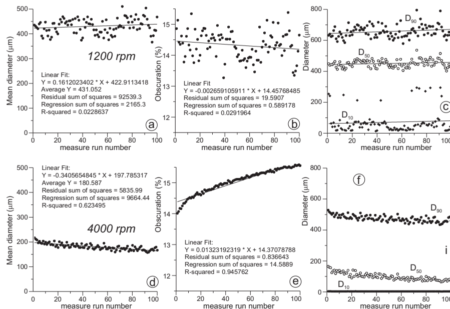
Fig. 9. Comparison between measure precision test results performed on sample CABRE3 at the pump speed test corresponding to the mean diameter peak value of the pump speed test (Fig. 3a), and at the maximum pump speed, respectively. (a) Test MP1200 5 performed on sub-sample aliquot CABRE3e by the Hydro 2000 MU dispersion unit; mean diameter value evolution with increasing the number of measurement runs. Data statistics is provided. (b) Laser obscuration value progression during the same test. Data statistics is provided. (c) Progression of D_{10} , D_{50} , and D_{90} percentiles during the same test. (d) Test MP4000 5 performed on sub-sample aliquot CABRE3f by the Hydro 2000 MU dispersion unit; mean diameter value evolution with increasing the number of measurement runs. Data statistics is provided. (e) Laser obscuration value progression during the same test. Data statistics is provided. (f) Progression of D_{10} , D_{50} , and D_{90} percentiles during the same test. Note the very large difference between the average mean diameter obtained from the first (431.052 μm) and the second test (180.587 μm), respectively. Both them are affected by strong recirculation-related mechanical bias.
