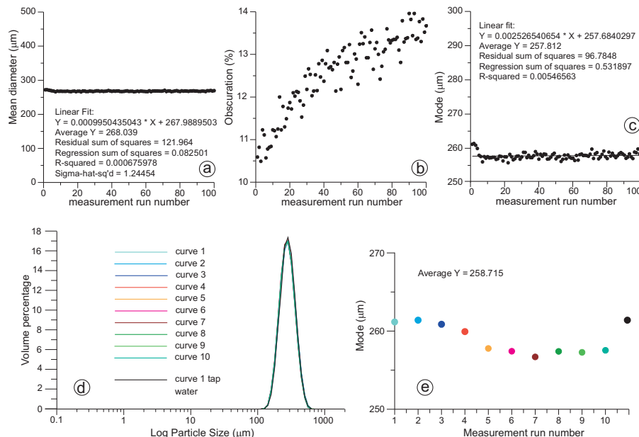
Fig. 17. Results of the chemical test MP2500 5a1 performed on sub-sample aliquot SAND1e by the Hydro 2000 MU dispersion unit, using denaturated ethylic alcohol as dispersant liquid. (a) Mean diameter value evolution with increasing the number of measurement runs. Data statistics is provided. (b) Laser obscuration value progression during the same test. (c) Progression of modal values with increasing the number of measurement runs. Data statistics is provided. (d) Granulometric curves computed for the first 10 runs, compared with the first curve from the test MP2500 5 on sub-sample aliquot SAND1c (Fig. 7). (e) Modal values corresponding to the curves in (d).
